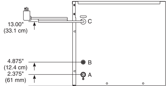
Front view — water-cooled RIDE model
