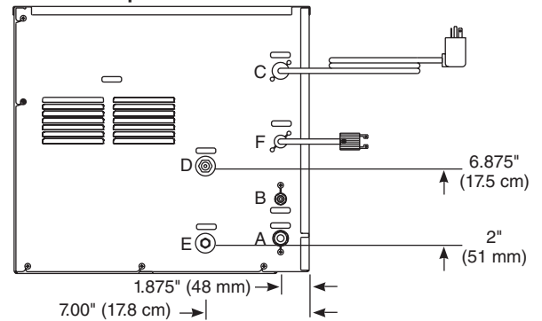
Back view — water-cooled top mount
