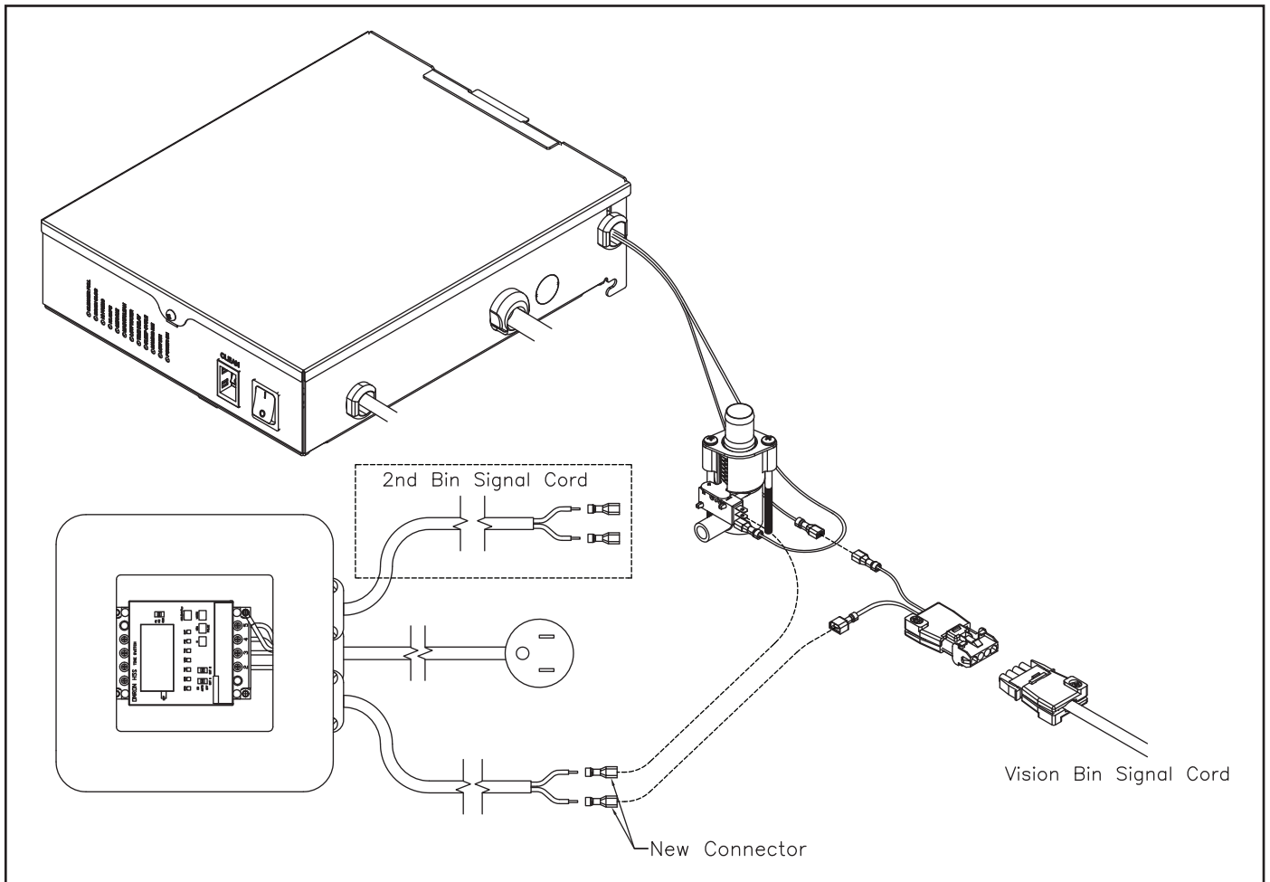
Fig. 2 Horizon 700, Horizon Elite 1010/1410 Vision Timer (Vision applications)
