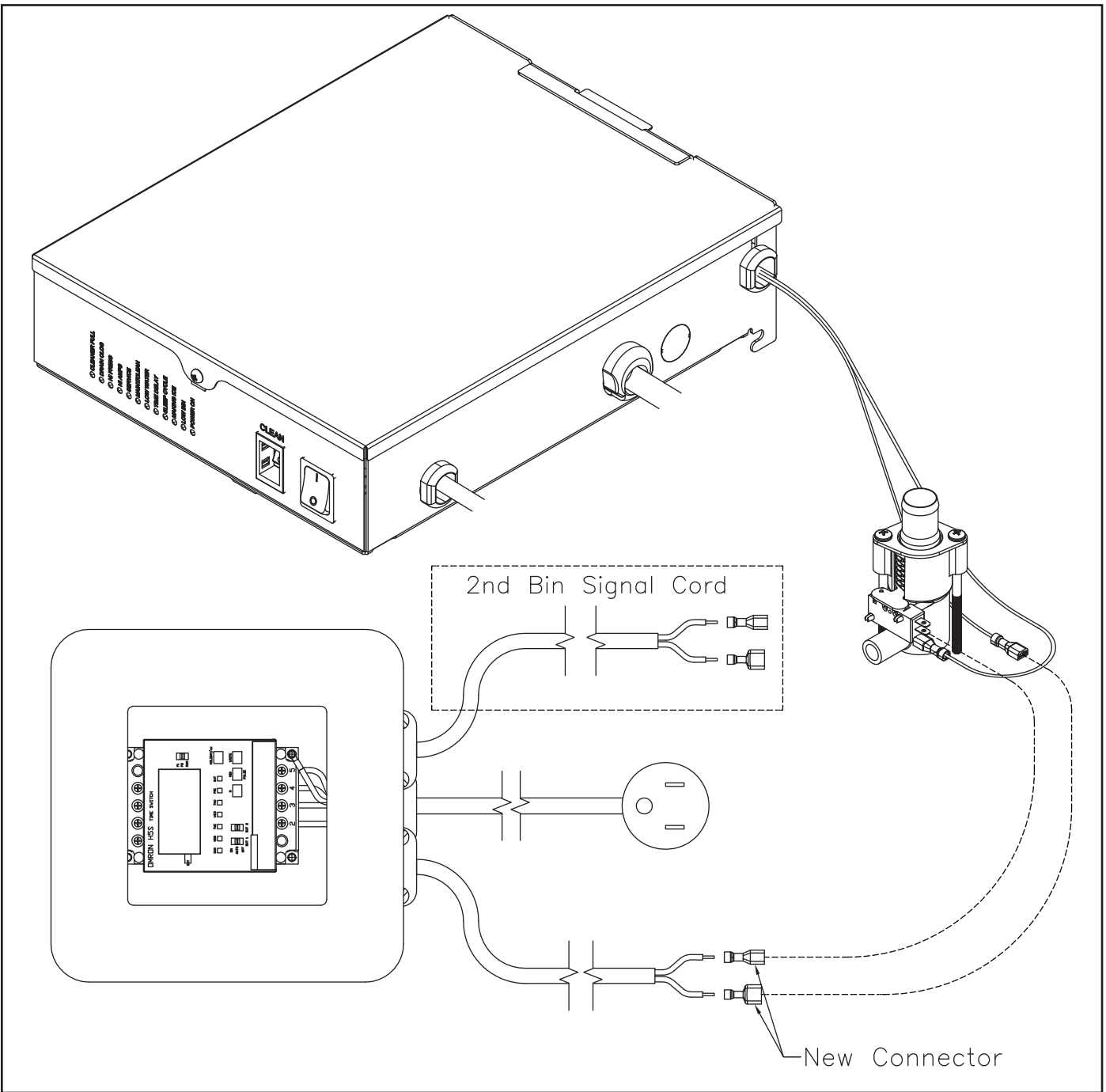
Fig. 1 Horizon 700, Horizon Elite 1010/1410 Timer (all applications except Vision)
