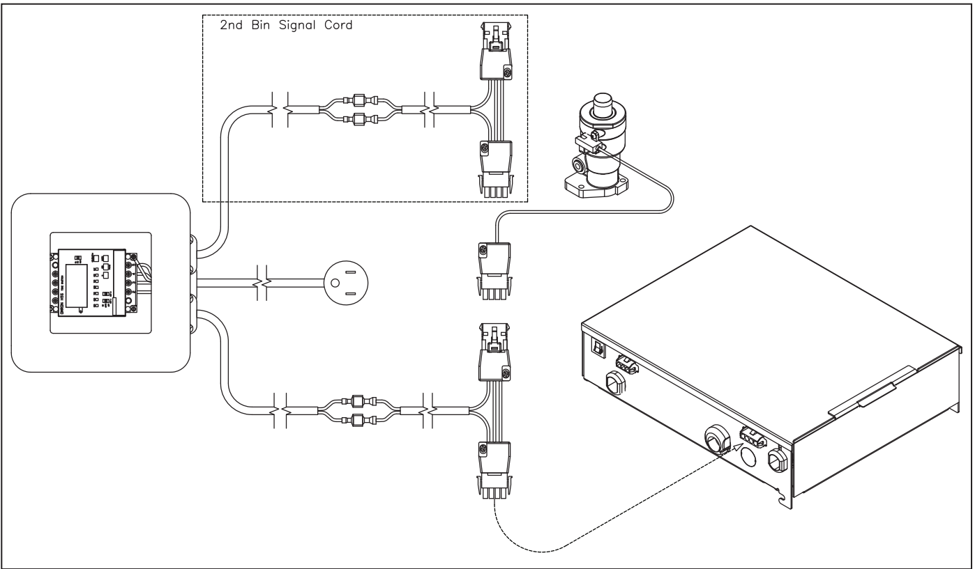
Fig. 3 Horizon 1000/1400/1650 Timer (all applications)
