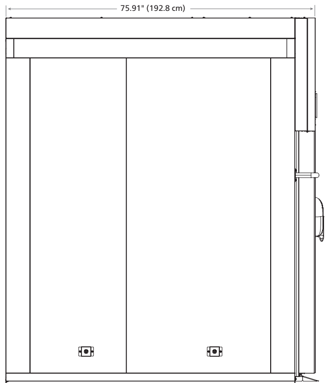
Side View
