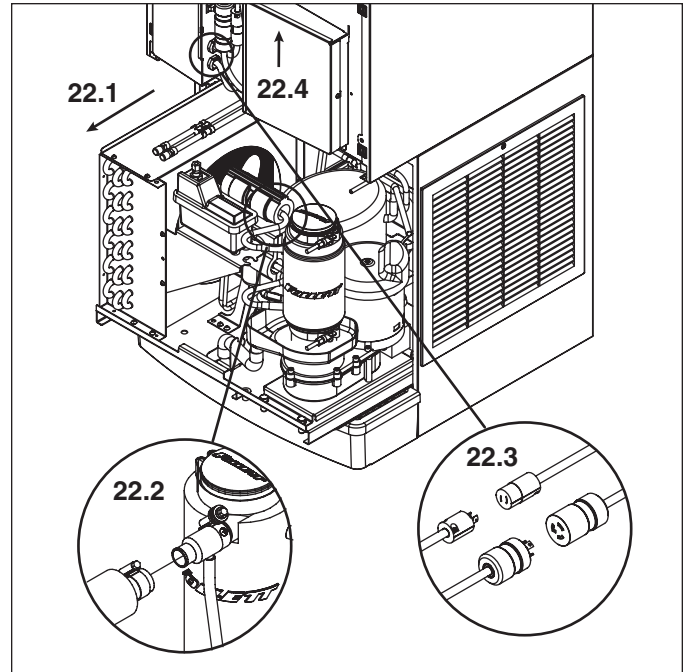
Fig. 22 – All models
