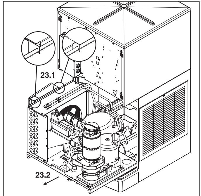
Fig. 23 – Air-cooled only
