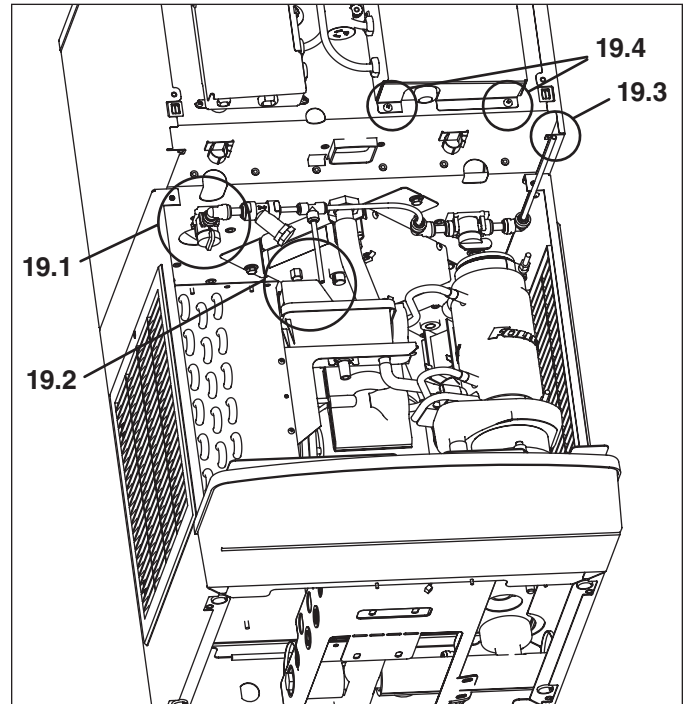
Fig. 19 – All models
