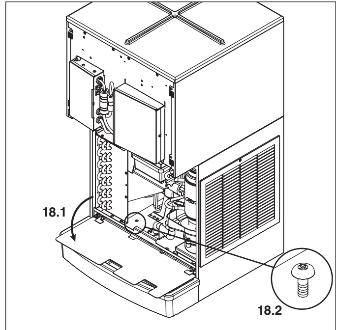
Fig. 18 – All models
